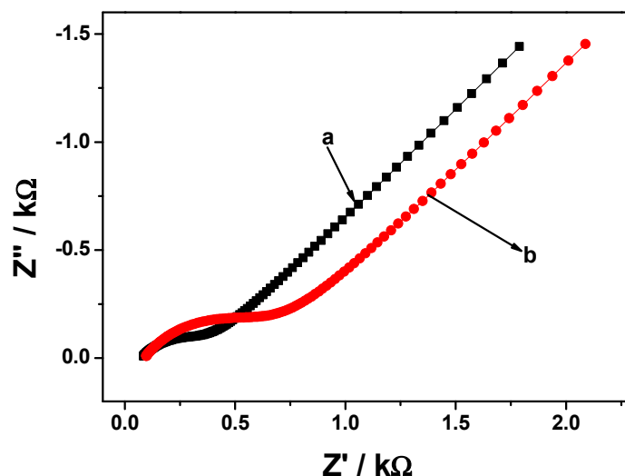
Figure 8. Nyquist plots of GCE/PT-PDMA-MWCNT after antibody immobilisation (curve a) and after immobilisation and blocking with BSA (curve b) in solution of 3 \times 10^{-5} \mu\text{M} of FB 1 .
