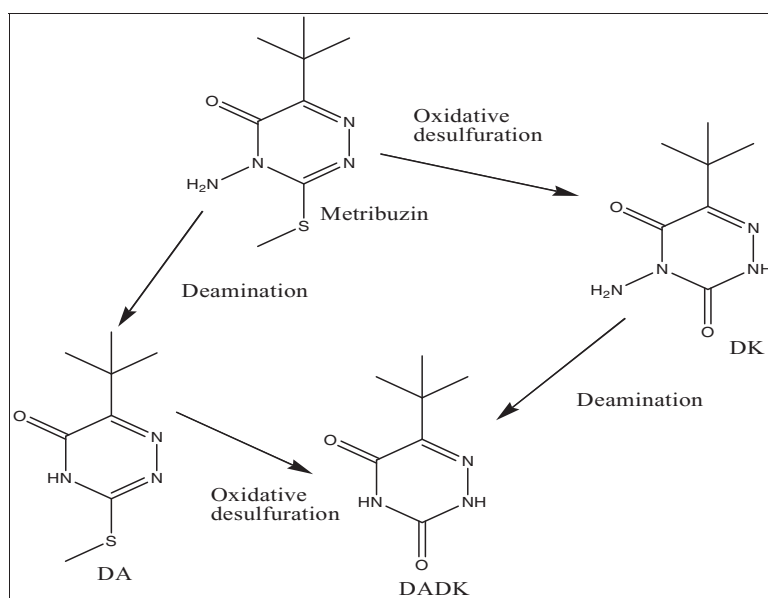
Figure 4. Degradation pathways of metribuzin (Huertas-Pérez et al. 2006).
