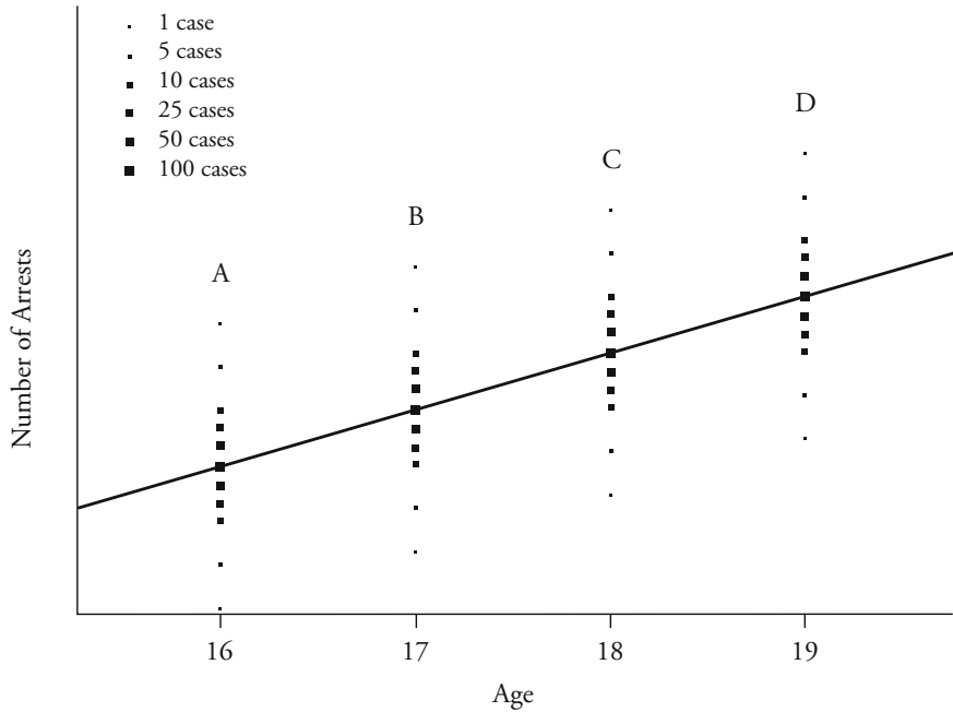
Scatterplot Showing Normal Distribution and Homoscedasticity
