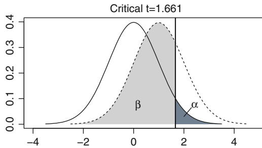
Graphical Representation for Power Analysis of a Correlation
