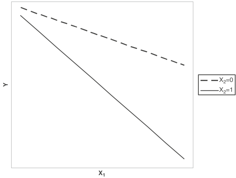
(d) b_1 and b_3 are both negative
