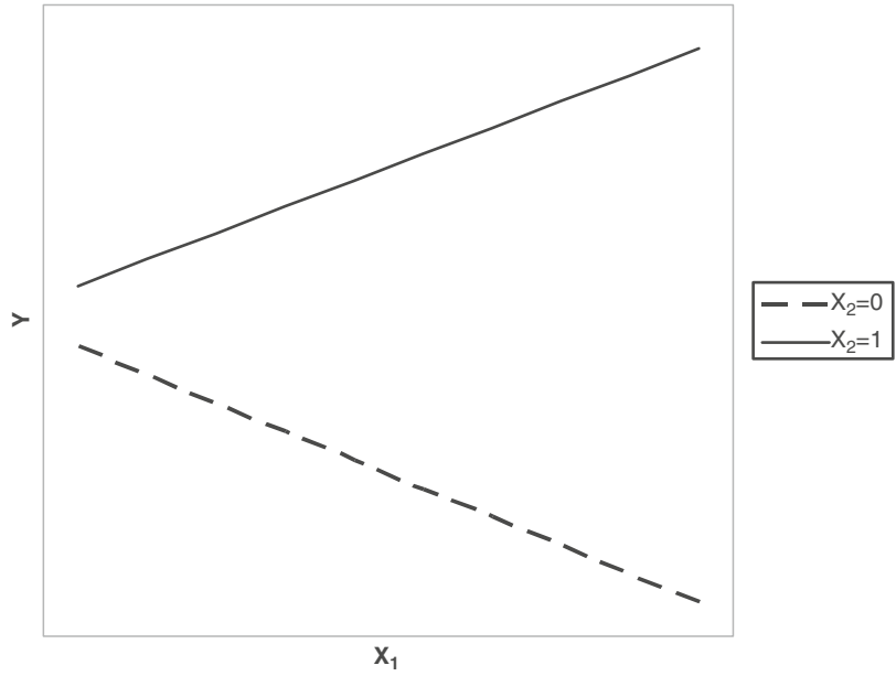
(c) b_1 is negative and b_3 is positive
