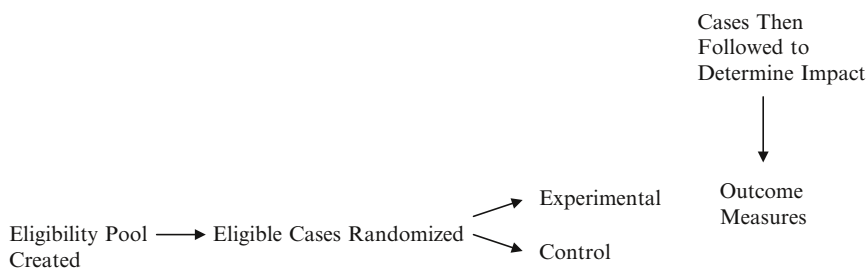
Diagram of the Typical Criminological Experiment
