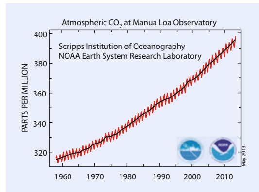
■ Fig. 23.2 Keeling curve (Courtesy NOAA)
