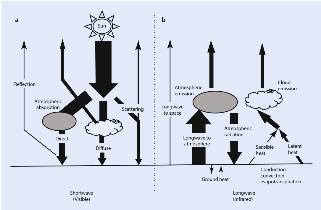
■ Fig. 15.2 Disposition of incoming solar radiation. Short wave radiation is high energy incoming photons and long wave radiation is outgoing (Source: Amy Chen)
