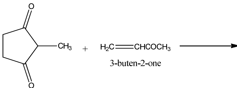
2-methyl- 1,3-cyclopentanedione
