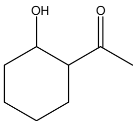
1-(2-hydroxycyclohexyl)ethan-1-one
