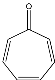
cyclohepta-2,4,6-trienone
