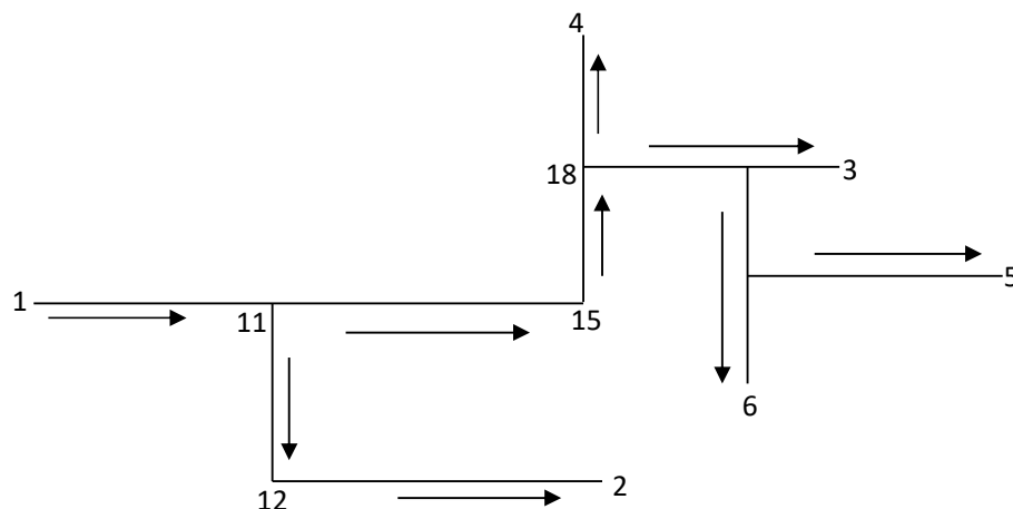
Figure 1: minimum paths tree connecting zone centroid 1 with zone centroids 2, 3, 4, 5 and 6 (8Marks)
