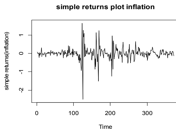
Figure 3.3 Simple returns
