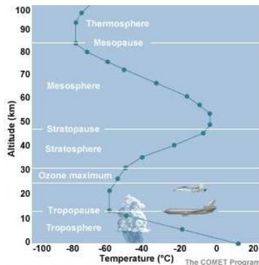
Figure 1; Variation of temperature with altitude
